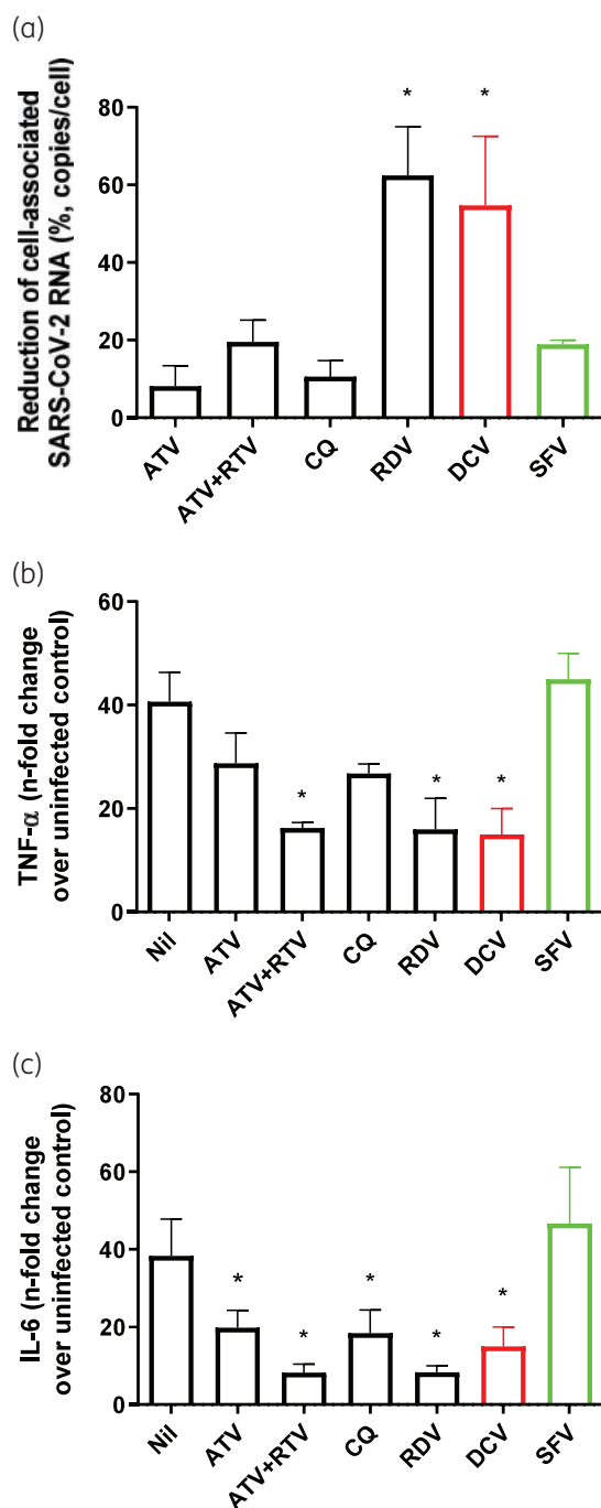
Figure 3. Daclatasvir impairs SARS-CoV-2 replication and cytokine storm in human primary monocytes. Human primary monocytes were infected at an MOI of 0.01 and treated with 1 \mu M daclatasvir (DCV), sofosbuvir (SFV), chloroquine (CQ), remdesivir (RDV), atazanavir (ATV) or atazanavir/ritonavir (ATV+RTV). After 24 h, cell-associated virus RNA loads (a) as well as TNF- \alpha (b) and IL-6 (c) levels in the culture supernatant were measured. The data represent means \pm SEM of experiments with cells from at least three healthy donors. Differences with P < 0.05 are indicated with an asterisk, when compared with untreated cells (Nil) for each specific treatment. This figure appears in colour in the online version of JAC and in black and white in the print version of JAC.
