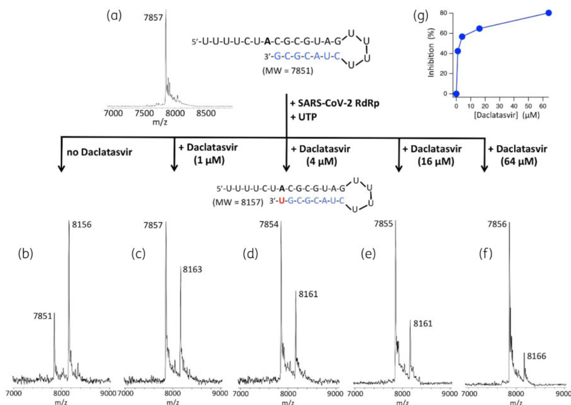
Figure 6. Inhibition of SARS-CoV-2 RdRp complex catalysed reaction by daclatasvir. A mixture of 500 nM RNA template-loop-primer (shown at the top of the figure), 1 μM SARS-CoV-2 pre-assembled RdRp complex (nsp12/nsp7/nsp8) and 3 μM UTP were incubated in buffer solution at 30°C for 1 h in the absence (b) or presence of daclatasvir at 1 μM (c), 4 μM (d), 16 μM (e) and 64 μM (f). The RNA template-loop-primer (a) and the products of the polymerase extension reaction (b–f) were analysed by MALDI-TOF MS. The signal intensity was normalized to the highest peak. The accuracy for m/z determination is \pm 10 Da. Reaction conditions were selected to yield an incorporation efficiency of approximately 70% as seen by MALDI-TOF-MS analysis in (b). The peak at 7851 Da corresponds to the RNA template-loop-primer (7851 Da expected) and the peak at 8156 Da corresponds to the U extended RNA product (8157 Da expected). Addition of daclatasvir reduced the amount of the U extended RNA product in a concentration-dependent manner. A plot for the inhibition of the polymerase reaction versus the daclatasvir concentration is shown in (g). This figure appears in colour in the online version of JAC and in black and white in the print version of JAC.
